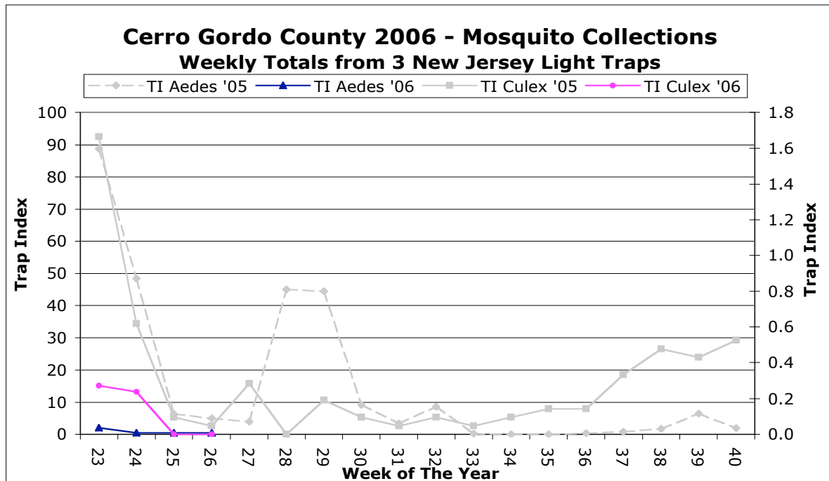
Figure 1. Aedes and Culex mosquito population levels according to trap index (TI=total mosquitoes trapped/total trap nights)
